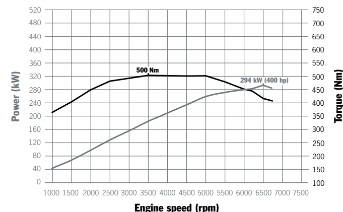
V8 engine
